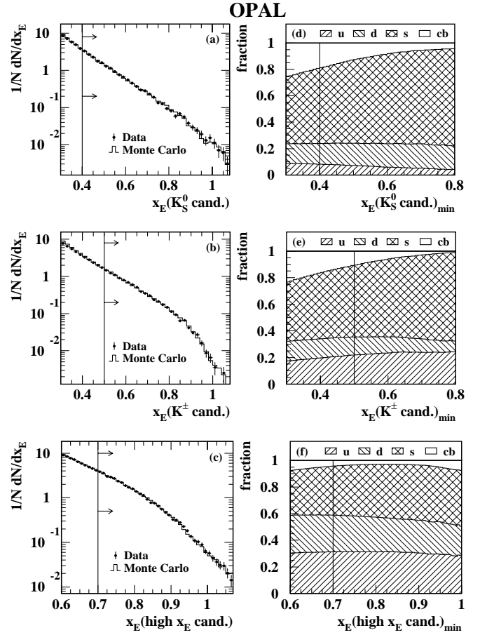
Fig. 1. a-c Observed energy spectra of K_S^0 , K^\pm , and high x_E candidates. The solid line shows the Monte Carlo simulation normalized to the integrated luminosity of the data after applying the reweighting procedure described in Sect. 3.4. d-f Corresponding flavour fractions taken from the Monte Carlo simulation as a function of the cut on the minimum energy fraction, x_{E,\text{min}} , of the tag particle. The x_E cuts chosen for the flavour enriched samples are indicated by the vertical lines
