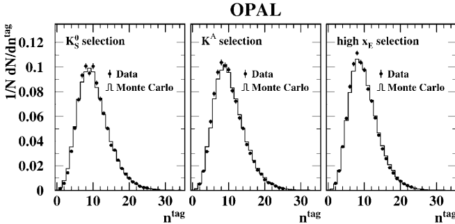
Fig. 3. Charged multiplicity distributions of the three selections, measured in the hemispheres opposite to the tag particles. Overlaid are the expectations from the Monte Carlo simulation
