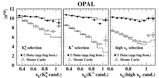
Fig. 2. Mean charged multiplicity in a hemisphere as a function of the energy of the tagged particles. Open circles show the values obtained from the hemispheres containing the tagged particle, full circles correspond to the opposite hemispheres. The histogram is the expectation from the Monte Carlo simulation
